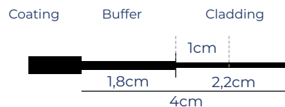
Cutting dimensions for CM SA connector
