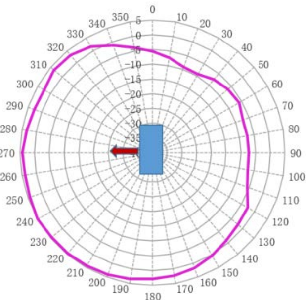
5.5G Wi-Fi XY plane (antenna2,3)
